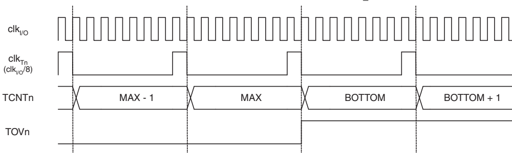
Figure 11-6. Timer/Counter Timing Diagram, with Prescaler ( f_{\text{clk\_I/O}}/8 )
