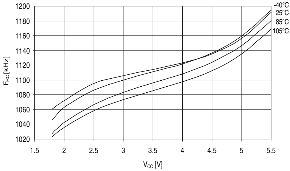
Figure 32-218. ATmega329PA - 105°C: Watchdog Oscillator Frequency vs. V CC
