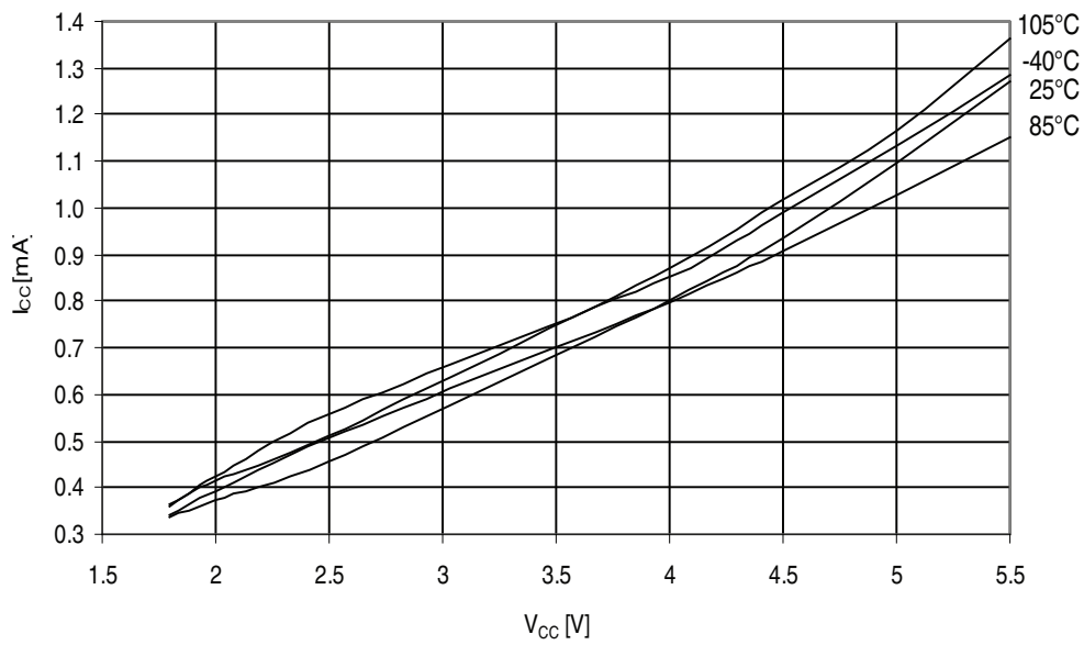
Figure 32-240. ATmega3290A - 105°C: Active Supply Current vs. V_{CC} (Internal RC Oscillator, 1 MHz)S
